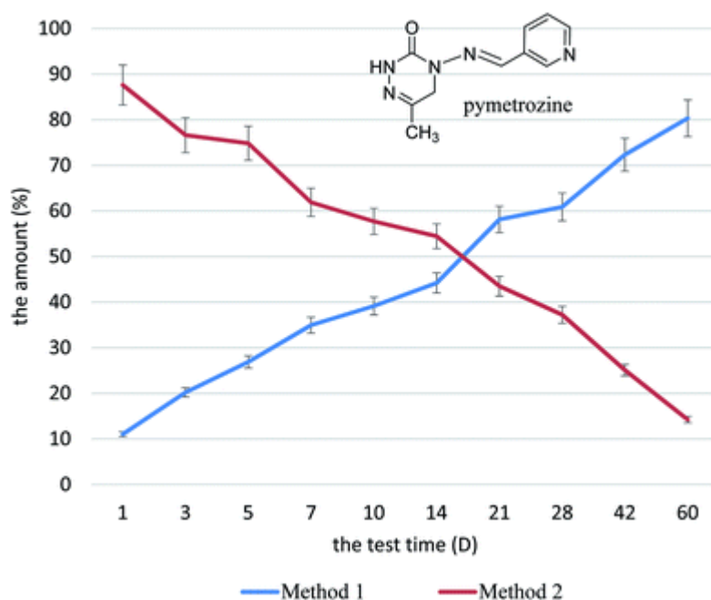
Fig. 1 The cumulative release of pymetrozine (%) from resin-based CRG at different designed to measure the amount of cumulative release amount (%) from the granule by pymetrozine in water at different time (day). Method 2 was designed to measure the amount remaining in the granule at different time (day).
